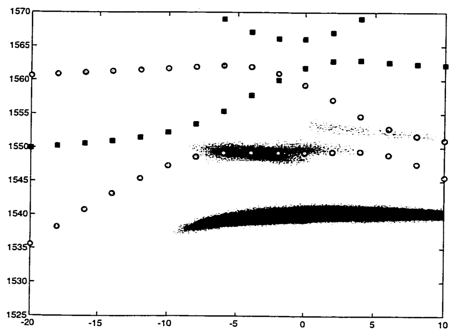
Figure 3.15: Calculated E_{\mu LH_v} light-hole exciton energies overlaid on experimental PL. There are no fitting parameters.
