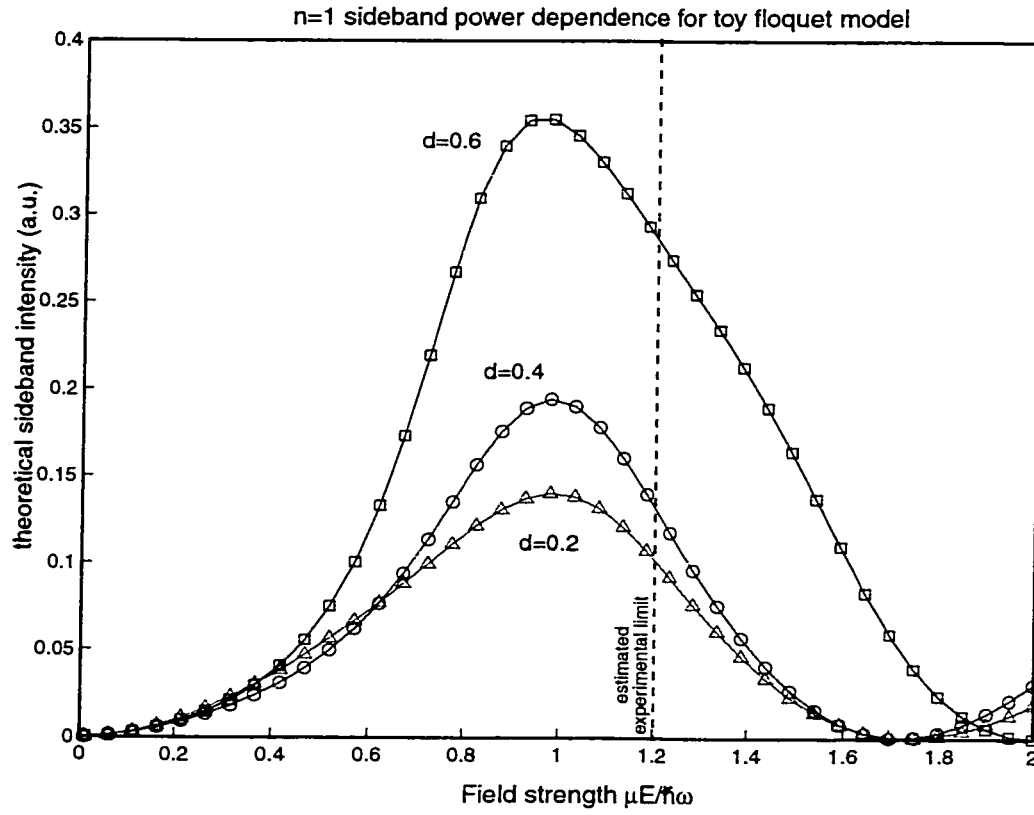
Figure 5.6: Sidebands calculated by evaluating (5.2.15) at various detuning parameters d = \frac{E_2 - E_1}{\hbar \omega} = 0.2, 0.4, 0.6 . Compare the results of this simplistic toy 3-level model with the experimental results of Fig. 5.4b.
