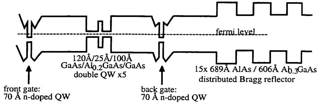
Figure 2.1: Sample band structure, containing frontgate, active region, backgate, and distributed Bragg reflector. Not to scale.
