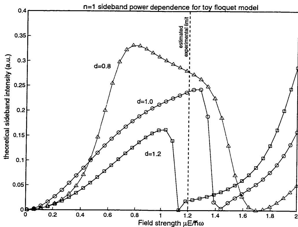
Figure 5.5: Sidebands calculated by evaluating (5.2.15) at various detuning parameters d = \frac{E_2 - E_1}{\hbar\omega} = 0.8, 1.0, 1.2 . Compare the results of this simplistic toy 3-level model with the experimental results of Fig. 5.4a.
